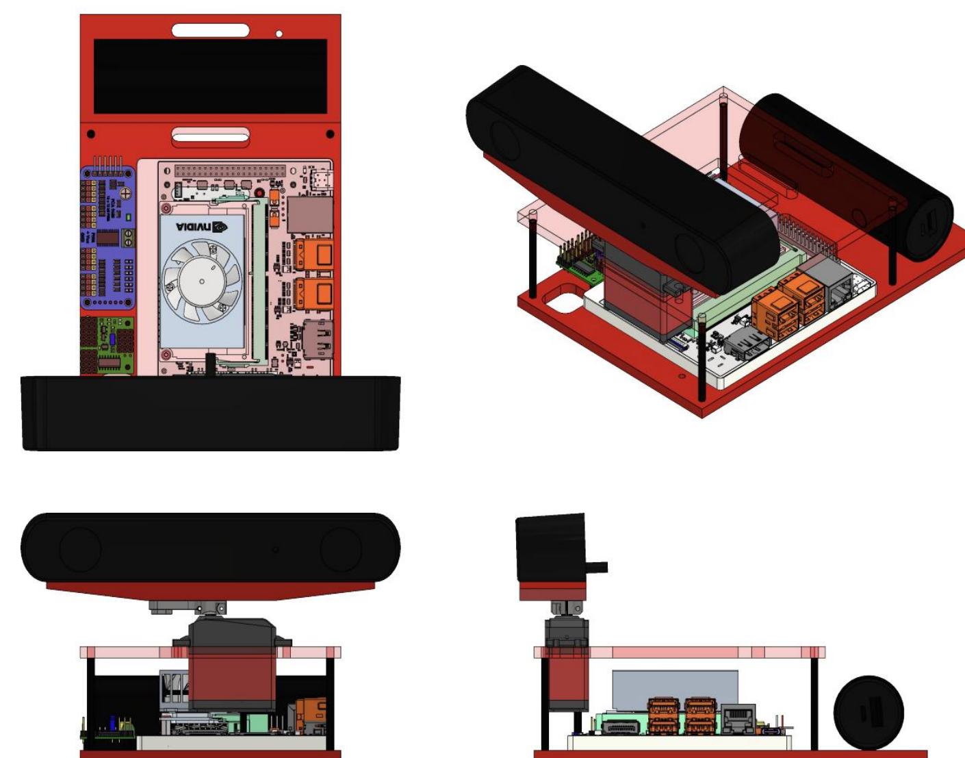
Fig 1. Hardware CAD
