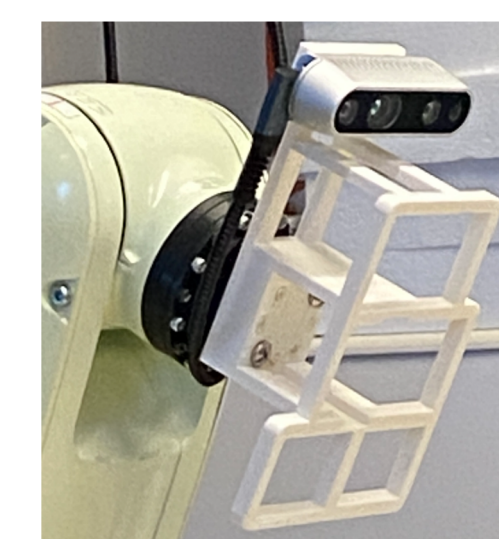
Fig. 1: Connector Plate Attached to Kawasaki Robot Arm
