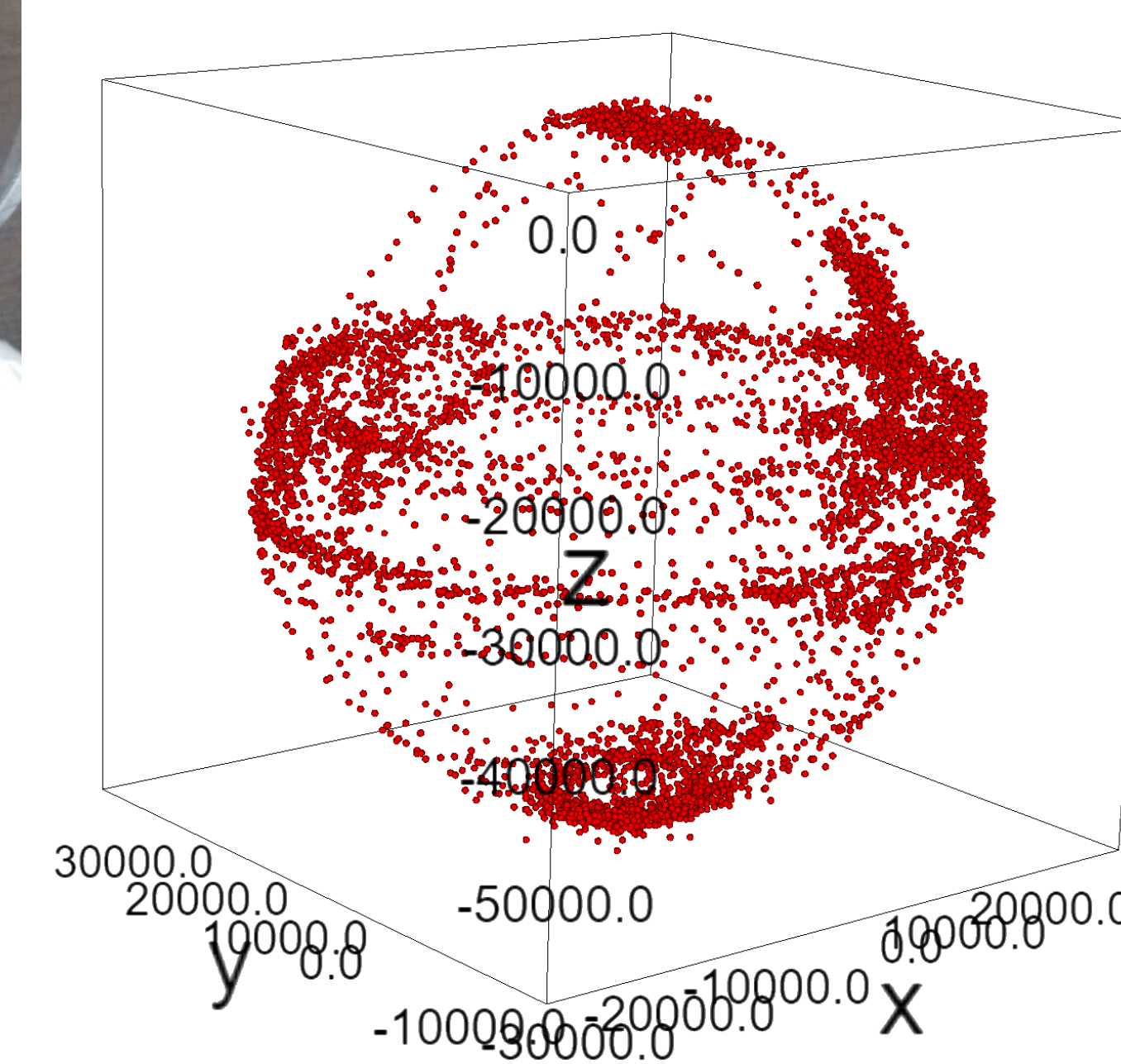
Raw magnetometer data (units in nanoTesla)
